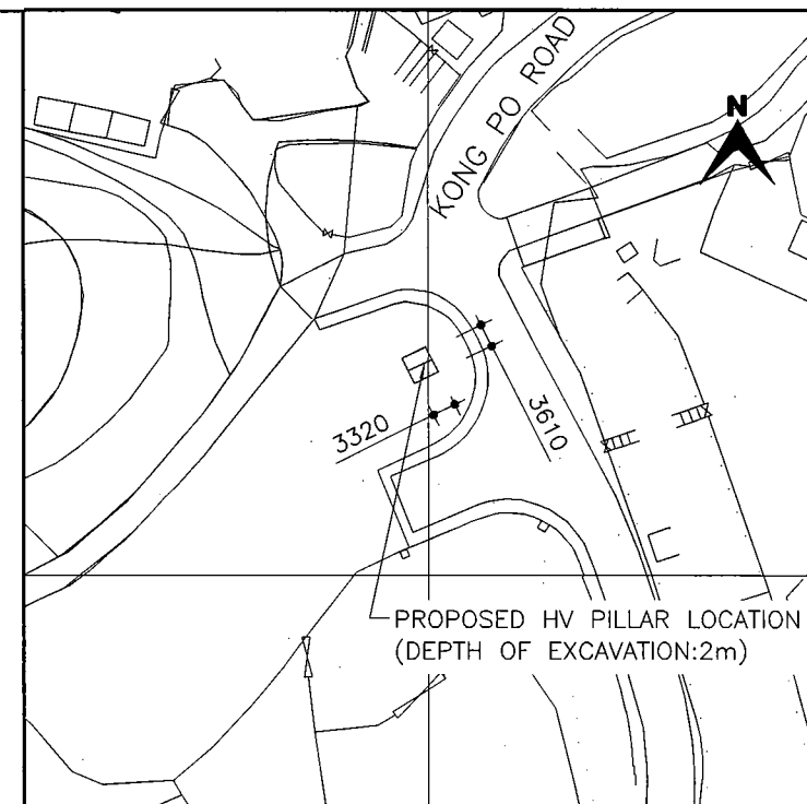
BLOCK PLAN SURVEY MAP No. 02SE108 SCALE = 1 : 1000
